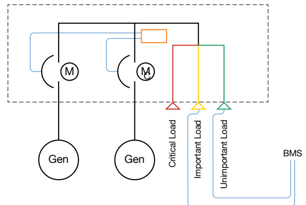
Figure 3: Parallel Generators with Load Management System (LMS)
