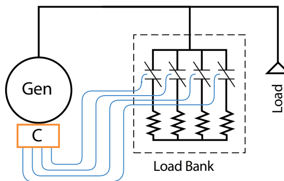
Figure 6: Single-Generator with Special Emission Requirements
