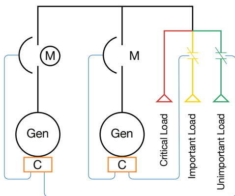
Figure 4: Parallel Generators with Load Management in Controller
