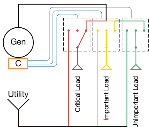
Figure 5: Single-Generator Controlling ATS
